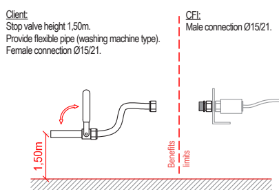
connection principles
